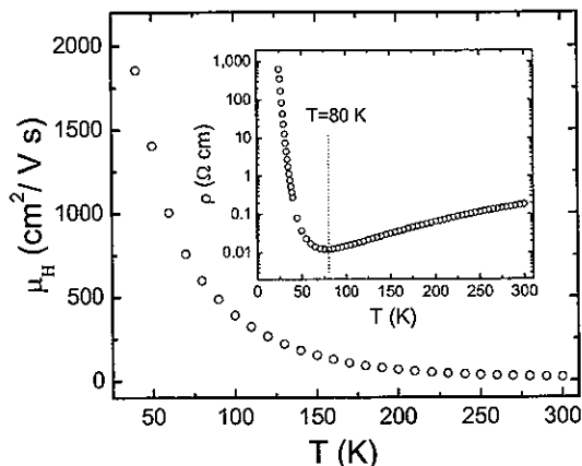
Figure 2. Temperature dependence of the Hall mobility for an Sb-doped ZnO film. The inset shows the temperature dependence of electrical resistivity.
